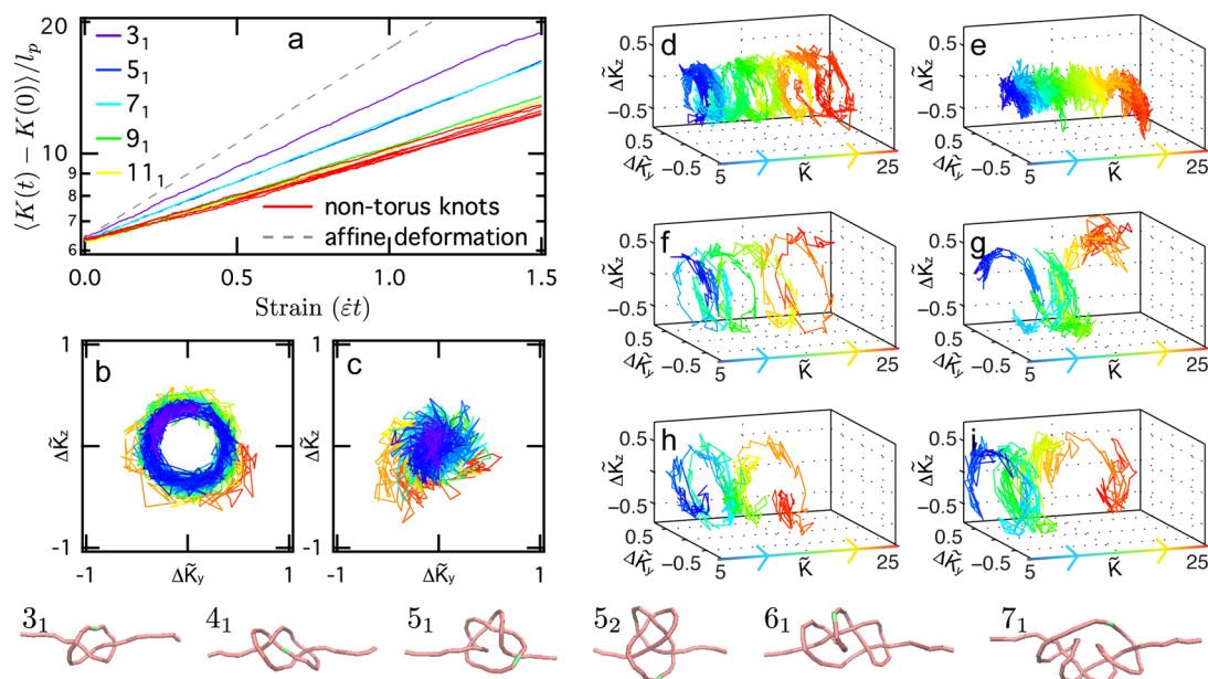
Figure 3. (a) Average knot displacements are plotted vs strain for various knots at flow strength Wi = 16 for knots initialized off-center ( K(t=0) = 6l_p \gg l for all topologies). The nontorus knots consist of the following: 4_1 , 5_2 , 6_1 , 6_3 , 10_{28} , and 15n165258 . 42 Displacements from the knot center of mass of the central segment of the knot made dimensionless by l_p ( \Delta\tilde{K}_y and \Delta\tilde{K}_z ) for the 3_1 (b) and 4_1 (c) knots in the plane orthogonal to the extensional axis; color changes from blue to red as the knot moves off the chain. Displacements from the knot center of mass of the central segment of the knot ( \Delta\tilde{K}_y and \Delta\tilde{K}_z ) in the plane orthogonal to the extensional axis plotted versus knot position ( \tilde{K} = K/l_p ) for the 3_1 (d), 4_1 (e), 5_1 (f), 5_2 (g), 7_1 (h), and 6_1 (i) knots. Color changes from blue to red as the knot moves off the chain. Bottom: snapshots of knots in (d–i) with central segments highlighted in green.
