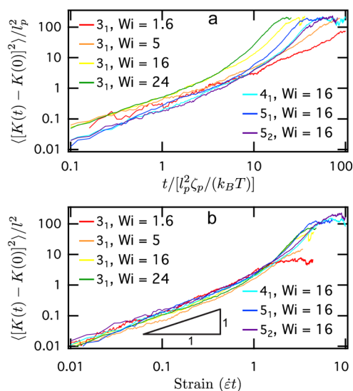
Figure 2. Mean squared displacements of initially centered knots ( K(t=0) = 0 ) in elongational flows. (a) Knot displacement plotted versus dimensionless time ( \zeta_p = n_p \zeta_b ). (b) Scaled knot displacement plotted versus strain. The triangle represents the slope of the diffusion-dominated mean squared displacement.
